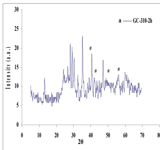
Fig. 2 (a) XRD patterns of GC-310-2h sample with \text{PbF}_2 phase (#).
