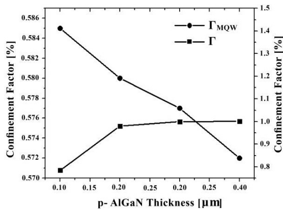
Fig. 7. \Gamma_{\text{MQW}} and \Gamma as the p-AlGaIn thickness.
