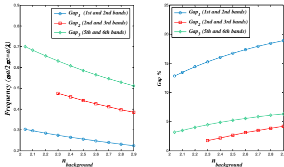
Fig. 5. Mid frequency of band gap versus background material index (Left) and relative photonic band gap versus background material index (Right) for considered 2-D 8-fold PQC.
