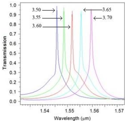
Fig. 8 The light power at port C with different values of n_L .
