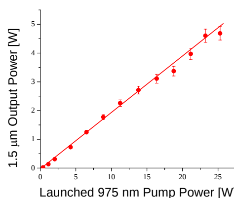
Fig. 1 Signal vs. launched pump power of a 3.5-cm phosphate PC fiber laser.
