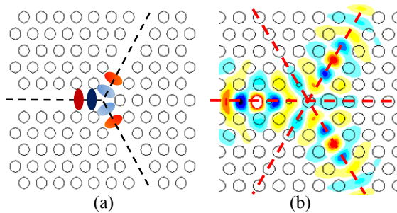
Fig. 9. The ideal resonance of a hypothetical Y-branch (b) The resonance profile obtained for the optimized Y-branch proposed in this paper for an input wavelength of 1550nm.
