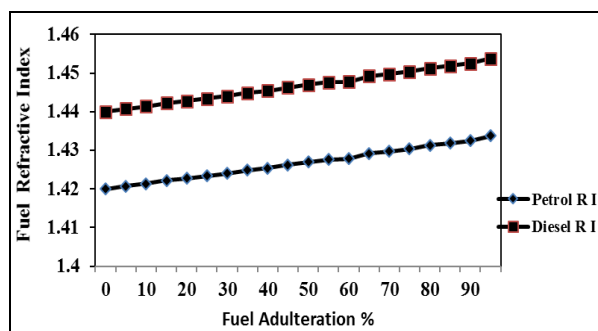
Fig. 7. Measured refractive index of adulterated fuel using Abbe's Refractometer.
