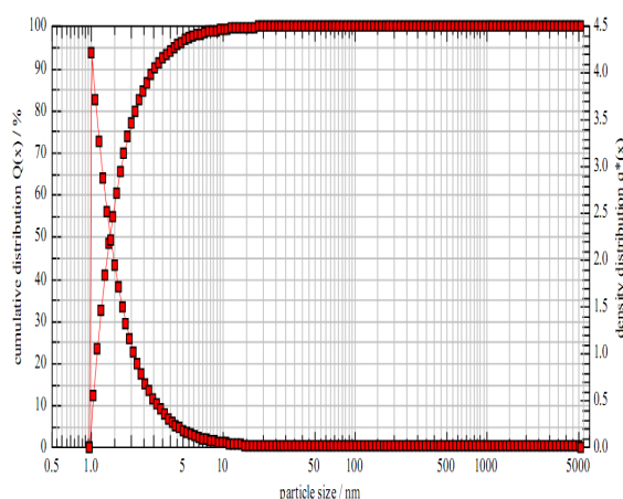
Fig. 10. Particle size distribution of compound 1 in a \text{CH}_2\text{Cl}_2 solution after green laser irradiation.
