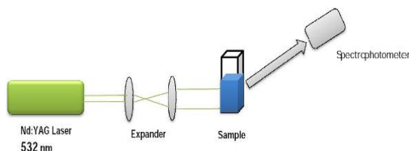
Fig. 1. Experimental set up for green laser irradiation.
