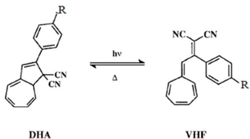
Fig. 1. photochromism in DHA-VHF (R=CN, OMe, Cl, NH 2 ).
