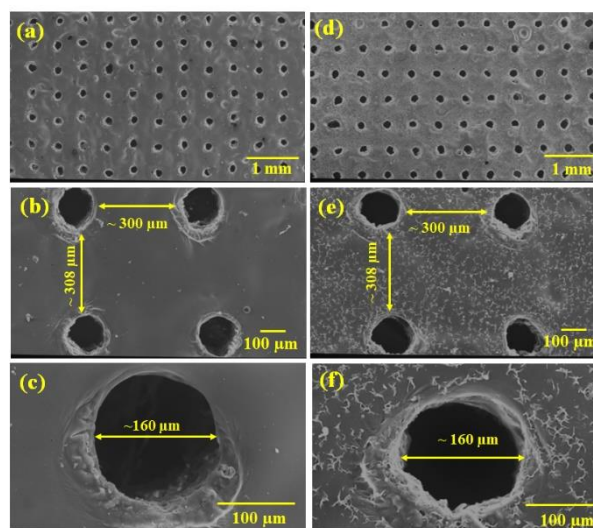
Fig. 3. SEM images of (a-c) PC-0.03TiO 2 mesh and (d-f) PC-0.03TiO 2 /ODA-90-laser.
