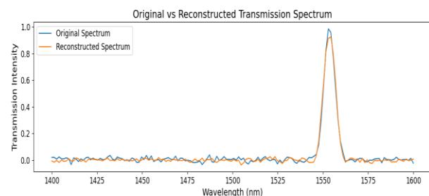
Fig. 4. Optical transmission spectrum reconstruction.
