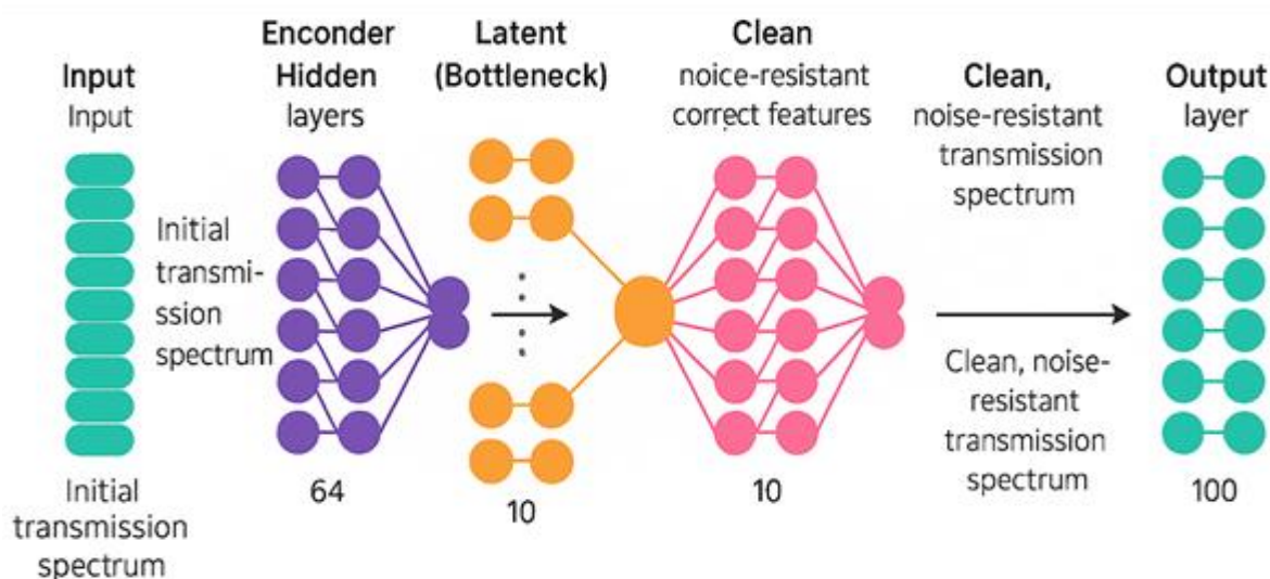
Fig. 1. Deep self-encoder architecture.
