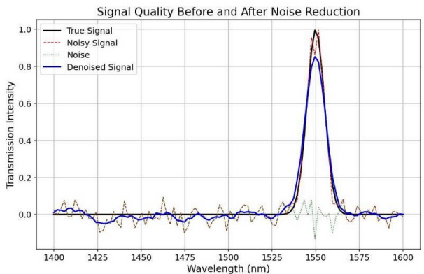
Fig. 7. Signal Transmission Spectrum: True, Noisy, Noise Component, and Denoised Signals Comparison.
