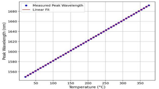
Fig. 6. Sensor Response: Peak wavelength shift as a function of temperature. Sensitivity (nm/°C): 0.4, Figure of Merit (FOM): 0.0004461170820581962, Limit of Detection (°C): 0.024999999999999998, R-squared of linear fit: 1.0.
