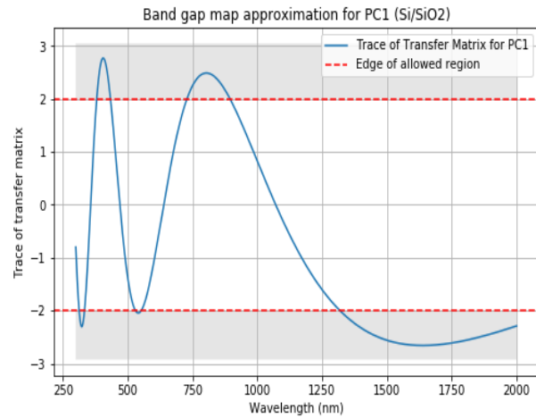
Fig. 3. Band gap for photonic structure.
