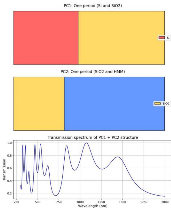
Fig. 2. Sensor structure and optical transmission spectrum.
