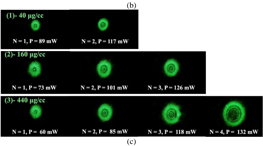
Fig. 3. SSPM diffraction ring patterns of hydraulic oil containing: (a) rGO, (b) rGO-OH, and (c) rGO-COOH in 40, 160, and 440 µg/cc concentration.
