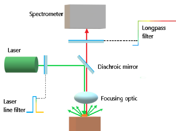
Fig. 3. Schematic diagram of the Raman spectrometer
