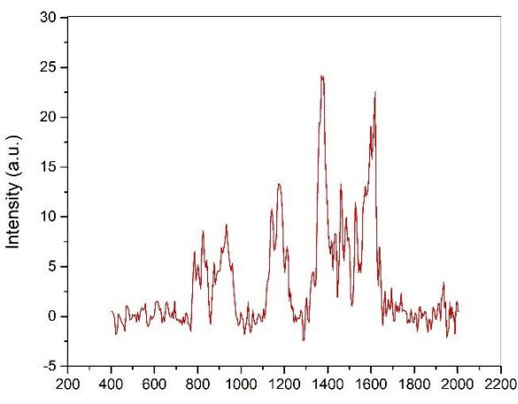
(b) Fig. 7. (a) Primary unsmoothed Raman spectrum and (b) baseline subtracted Raman spectrum of CV solution placed on a graphene-based substrate.
