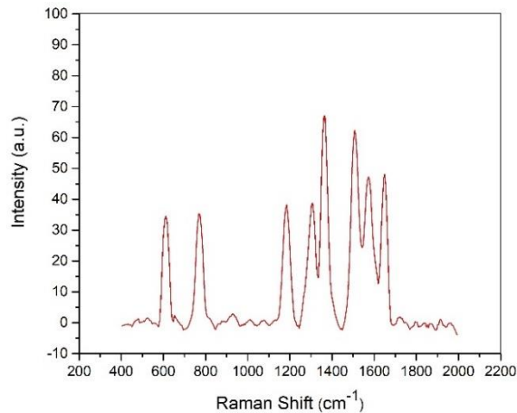
(b) Fig. 6. (a) Primary unsmoothed Raman spectrum and (b) baseline subtracted Raman spectrum of R6G solution placed on a graphene-based substrate.
