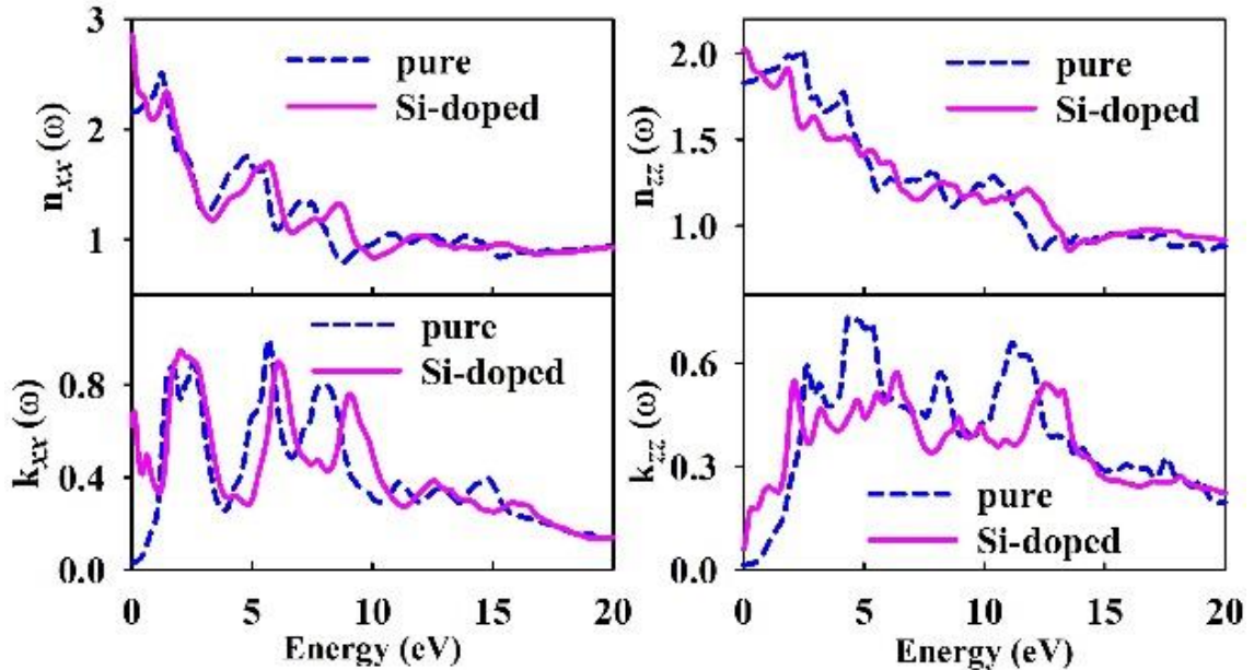
Fig. 6. xx-(left) and zz-components (right) of refraction (top) and extinction (bottom) functions of pure (dashed lines) and silicon-doped (solid lines) \text{Sc}_2\text{C}(\text{OH})_2 monolayer.
