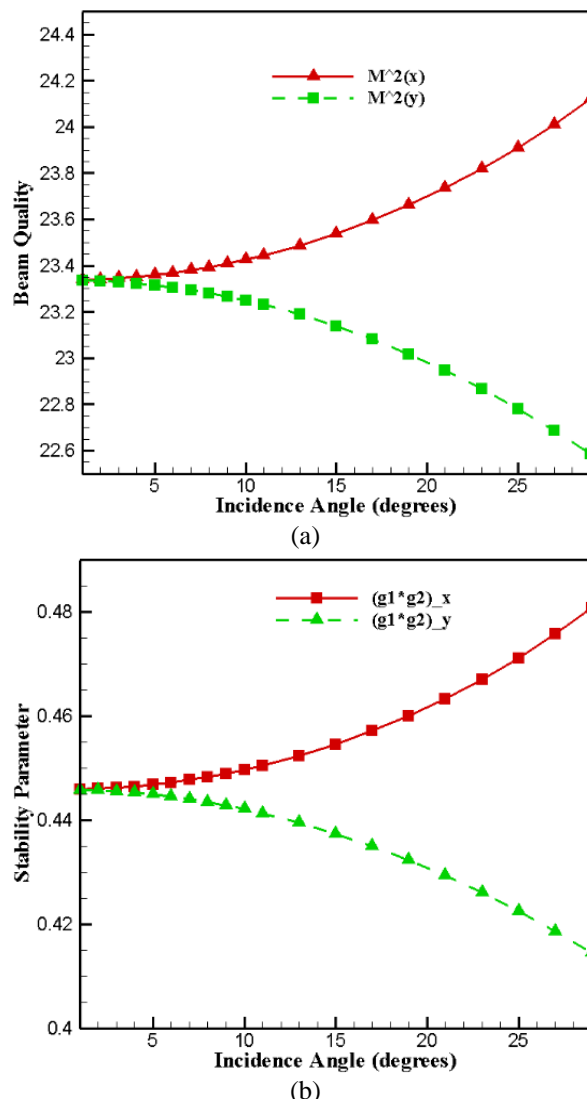
Fig. 9. The angle dependency of beam quality (a) and resonator stability (b) in V-shaped dumped cavity.
