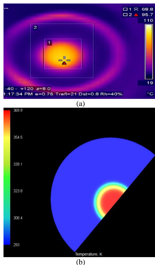
Fig. 12. (a) thermography of disk surface in maximum pump power and (b) simulation of temperature distribution of the disk surface.
