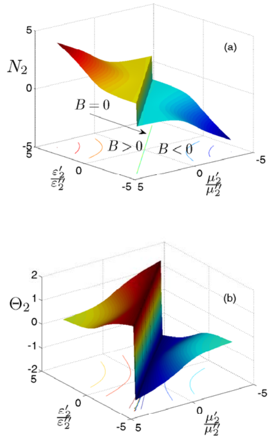
Fig. 3 (Color online) a) Real refractive index N_2 and b) real refraction angle \theta_2 as functions of \varepsilon_2'/\varepsilon_2'' and \mu_2'/\mu_2'' for n_1^2 \sin^2 \theta_1 / \varepsilon_2''\mu_2'' = 1 .
