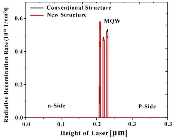
Fig. 15. Radiative recombination rates of the conventional and the optimized new quadruple asymmetric waveguide LDs.
