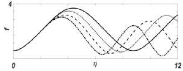
Fig. 3. Variation of beam width parameter, f , respect to propagation distance, \eta , at T_{e01} = 5\text{keV} for \alpha A_{00}^2 = 0.8\text{eV} , n_0 = 2.4 \times 10^{18}\text{cm}^{-3} , r_0 = 20\mu\text{m} , and \omega = 6.28 \times 10^{14}\text{s}^{-1} .
