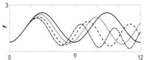
Fig. 4. Variation of beam width parameter, f , respect to propagation distance, \eta , at T_{e02} = 10\text{keV} for \alpha A_{00}^2 = 0.8\text{eV} , r_0 = 20\mu\text{m} ,
