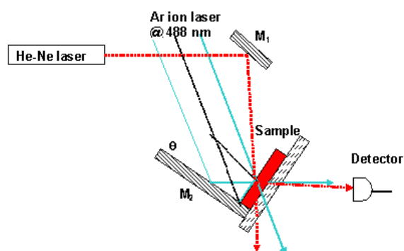
Fig. 5 Schematic diagram for the measurement of diffraction efficiency of the SRG in polymeric films. M_1 and M_2 are mirrors. The angle \theta is 10^\circ .
