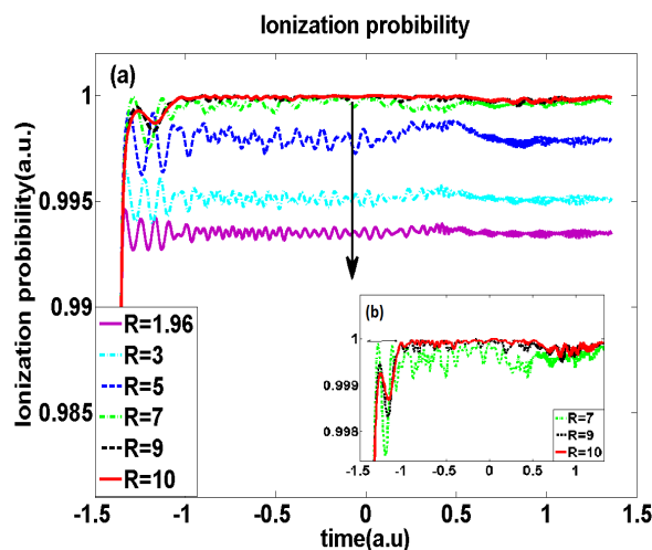
Fig. 4. (a). Variation of the ionization probability of the H_2^+ 1-D model electron with time at different inter-nuclear distances obtained under the influence of a three color laser pulse and (b). This figure is the zoom in case for R=7-10 .
