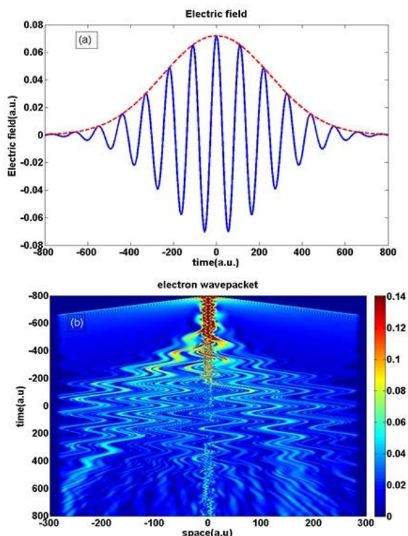
Fig. 3. (a). One color laser field (blue solid line) with a Gaussian envelope (red dashed line) and (b). Its corresponding wave packet for \tau = 10 fs .
