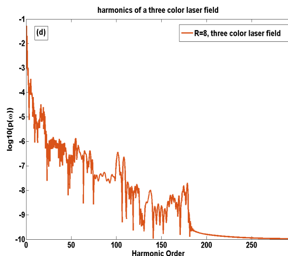
Fig. 5. High-order-harmonic spectra produced by H 2 + molecule under homogenous three color laser field at (a). R=1.96 (a.u.), (b). R=2 (a.u.), (c). R=5 (a.u.) and (d). R=8 (a.u.).
