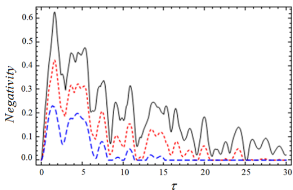
Fig. 4. Time evolution of negativity at temperatures of T = 0K (solid curve, black), T = 4K (small-dashed curve, red) and T = 8K (large-dashed curve, blue) for the initial mean photon number of \bar{n} = 2 .
