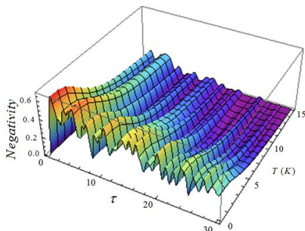
Fig. 7. Negativity versus scaled time, \tau , and temperature, T , for the case of an initial photonic
