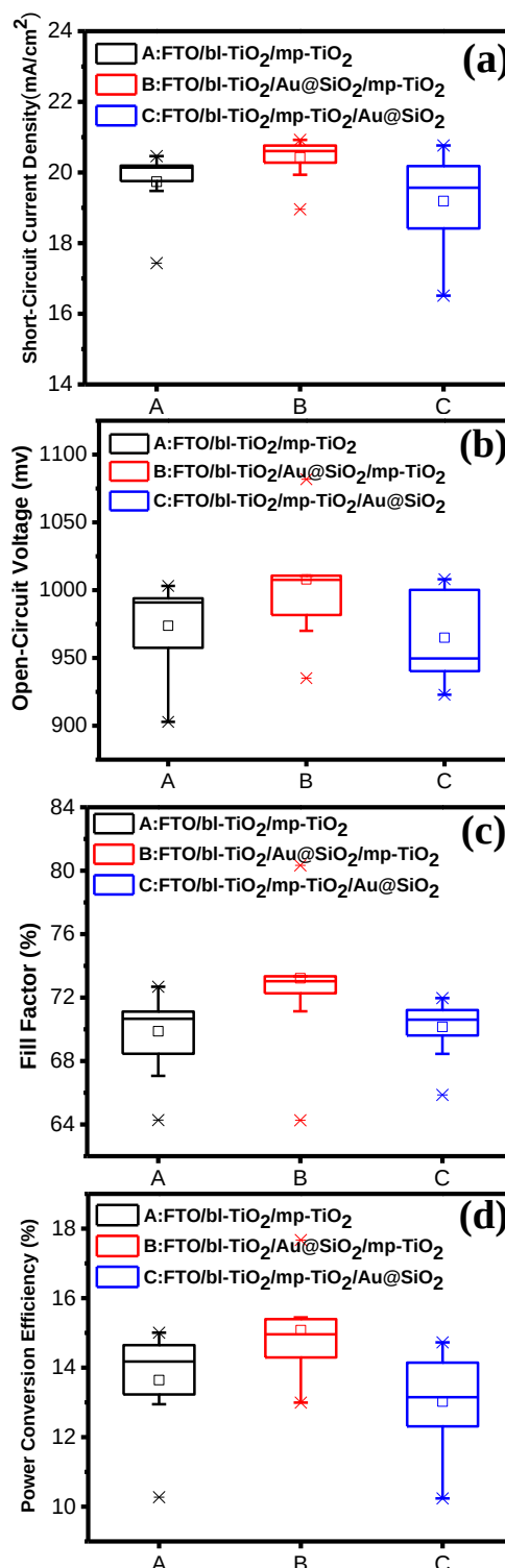
Fig. 7. Statistics parameters for the photovoltaic performance for 20 cells using different concentration of Au@SiO 2 (a) J_{sc} , (b) V_{oc} , (c) FF, (d) PCE. A:FTO/bl-TiO 2 /mp-TiO 2 , B:FTO/bl-TiO 2 /Au@SiO 2 /mp-TiO 2 , C:FTO/bl-TiO 2 /mp-TiO 2 /Au@SiO 2 .
