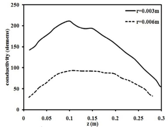
Fig. 8. Variation of the conductivity with respect to the axial positions at two different radial positions, i.e., r=0.003\text{m} (solid line) and r=0.006\text{m} (dashed line).
