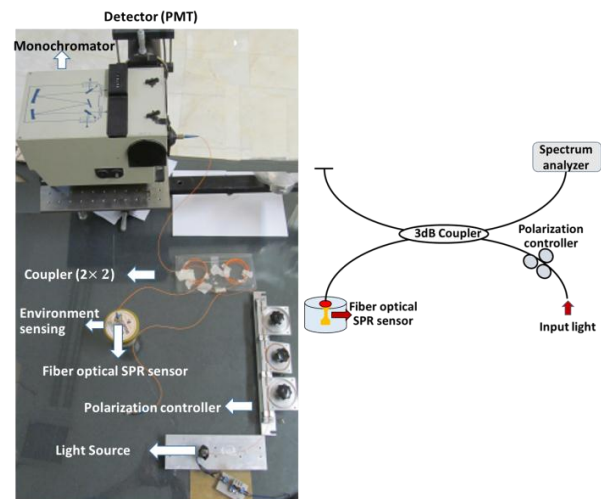
Fig. 8: the picture (left) of the sketched (right) experimental setup used to measure the lead concentration in water by fabricated fiber SPR sensor.
