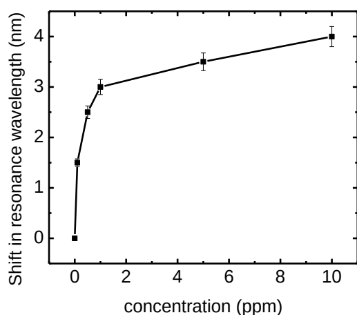
Fig. 10: The SPR wavelength shift versus concentration of lead in water.
