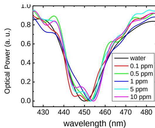
Fig. 9: measured spectra of the fiber SPR sensor for different concentrations of lead in water.
