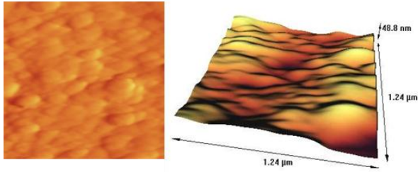
Fig. 7: AFM 3D (right) and 2D (left) images of an area of about 1.5 \mu\text{m}^2 of the taper after silver deposition.
