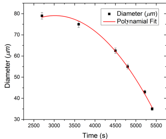
Fig. 5: Acidic etching rate of a multimode glass fiber (core/cladding-50/125 \mu\text{m} ) using HF acid with 49% purity when a 10 \mu\text{liters} droplet is used.
