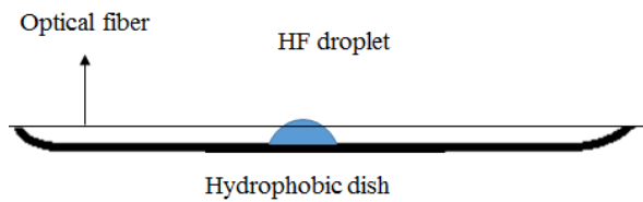
Fig. 1: Schematic of the etching method based on surface tension driven flows of hydrofluoric acid micro droplets to fabricate fiber optical taper.
