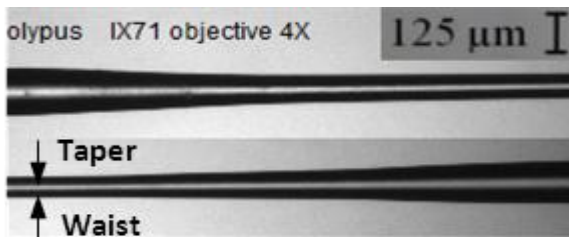
Fig. 4: The image of the fabricated taper under an optical microscope with a 4X objective. The minimum waist of the cone shape taper is about 40 \mu\text{m} .
