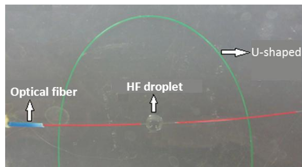
Fig. 3: Picture of the etching setup to make about 2 mm long fiber taper. The green U-shaped piece of an optical fiber is used to maintain the efficient reaction of the etching area with acid droplet.
