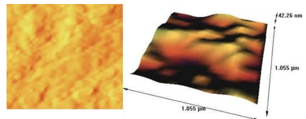
Fig. 6: Recorded 3D (right) and 2D (left) images of an area of about 1 \mu\text{m}^2 of the taper by AFM.
