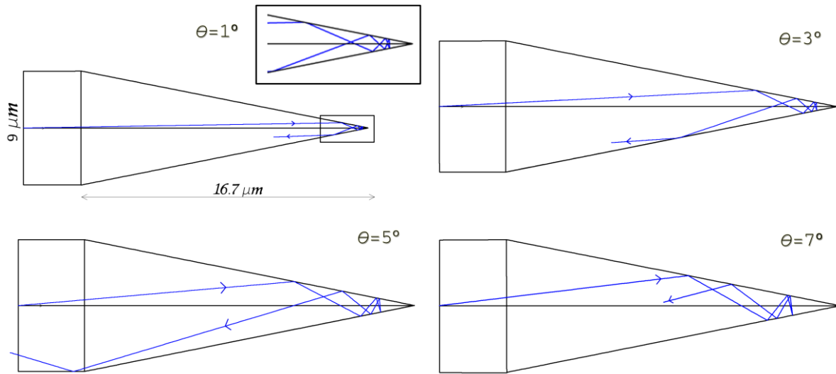
Fig. 5: Ray optic simulation of the fiber tip using ZEMAX for different incident ray angles (only core region is shown)
