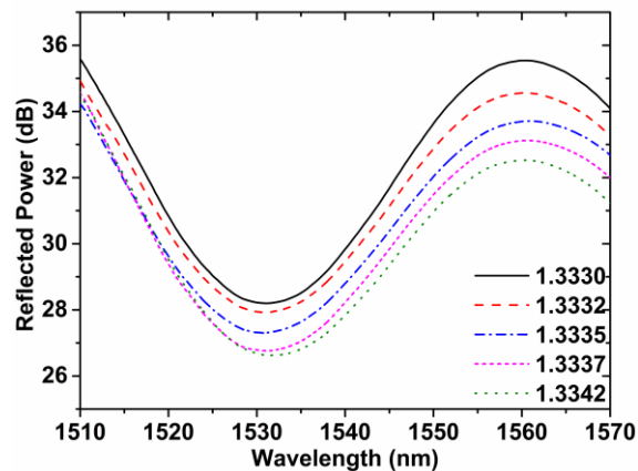
Fig. 6: Reflection spectrum of the probe in different RIs
