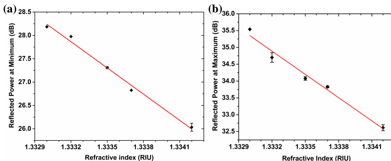
Fig. 7: Change in reflected power at minimum (a) and maximum (b) versus RI
