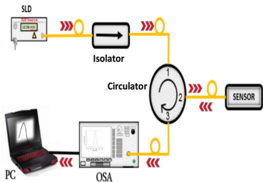
Fig. 3: Schematic experimental setup
