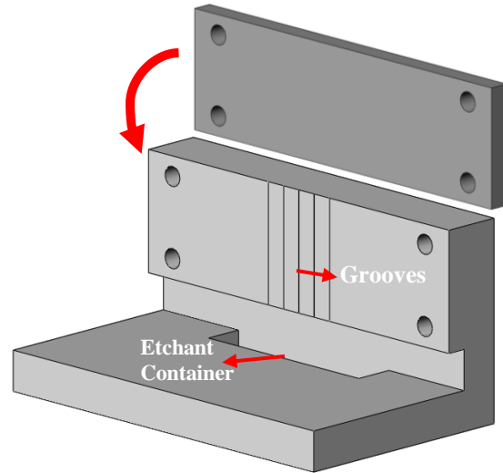
Fig. 2: The fiber holder for etching
