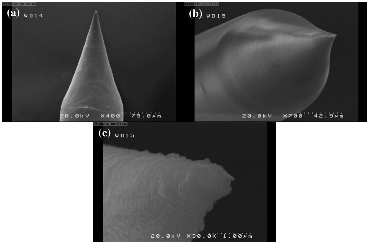
Fig. 4: SEM images of a tapered fiber tip made by using a modified etching method. (a) side view , (b) 3D view and (c) sub-micrometer tip aperture
